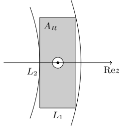
Figure 24: Deformation of the region A , which yields the same result in the \delta \rightarrow 0 limit.
