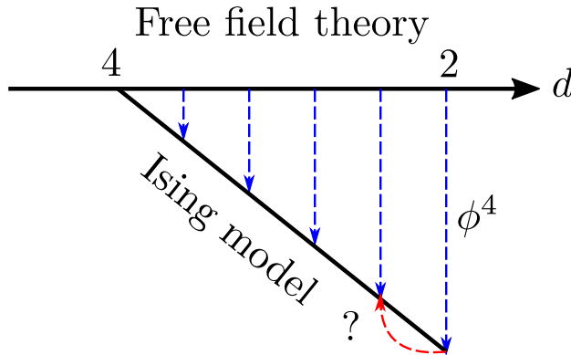
Figure 18: A standard RG flow diagram where long arrows are strongly coupled and short arrows are weakly coupled. In this case, we show the standard approach to the short-range Ising model where perturbation theory can only be done close to d = 4 despite the fact that d = 2 is a solved case as well. This is what the long-range RG flow diagram looked like before the work of [159, 160].
