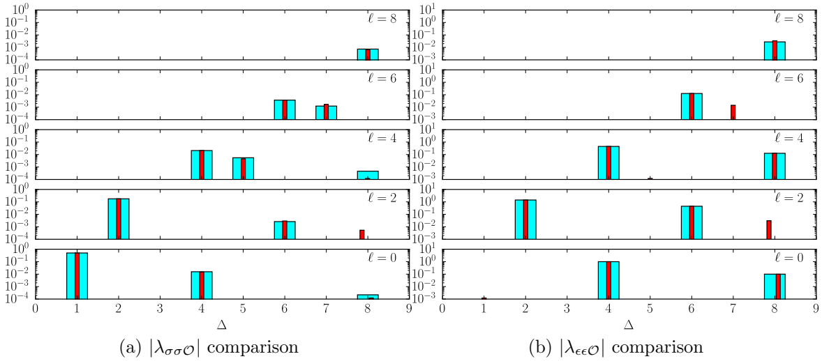
Figure 5: OPE coefficients in the 2D Ising model for operators with \Delta \leq 8 . Wide blue bars show exact values and narrow red bars show estimates from the fit used in [90].
