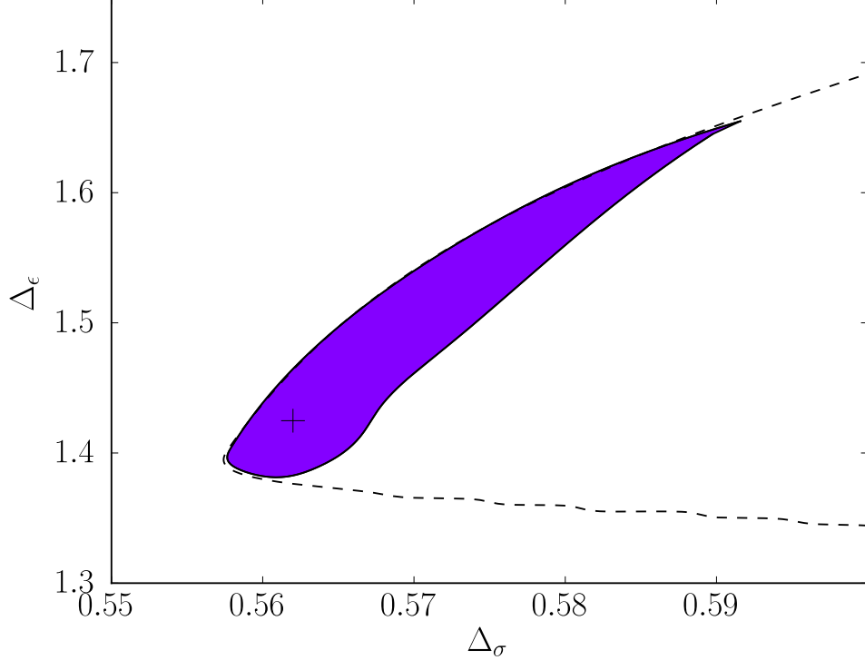
Figure 37: The island for the \Delta_T = 3.1 model computed with (m_{\max}, n_{\max}) = (3, 5) . Unlike Figure 34, which contains a much larger purple region for \Delta_T = 3.1 , this uses the full content of the shadow relation captured in the crossing equation (4.157) — i.e. it was obtained by demanding crossing symmetry and unitarity for the ansatz built out of the superblocks (4.158). An island only forms because of the superblocks and the fact that we are imposing a spin-2 gap above \Delta_T . In this case, the gap is \Delta_{T'} \geq 4.5 . The old \Delta_T = 3.1 region that would be produced from a bootstrap with ordinary conformal blocks and / or no \Delta_{T'} gap is shown with a dotted line for comparison.
