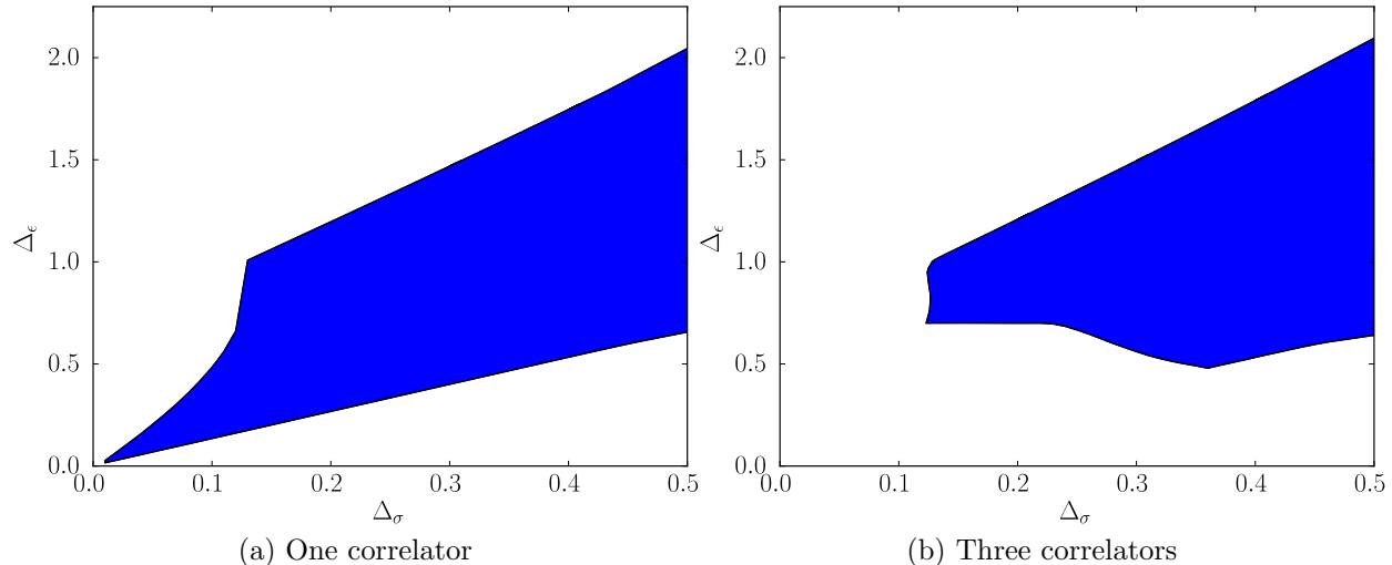
Figure 8: Allowed regions for the dimensions of \sigma and \epsilon — the \mathbb{Z}_2 -odd scalar of smallest dimension and the \mathbb{Z}_2 -even scalar of smallest dimension respectively. The left plot follows from the constraints of crossing symmetry and unitarity on the four-point function \langle\sigma\sigma\sigma\sigma\rangle . The right plot comes from the same constraints on \langle\sigma\sigma\sigma\sigma\rangle , \langle\sigma\sigma\epsilon\epsilon\rangle and \langle\epsilon\epsilon\epsilon\epsilon\rangle . In both cases, all OPEs are restricted to contain only one relevant scalar.
