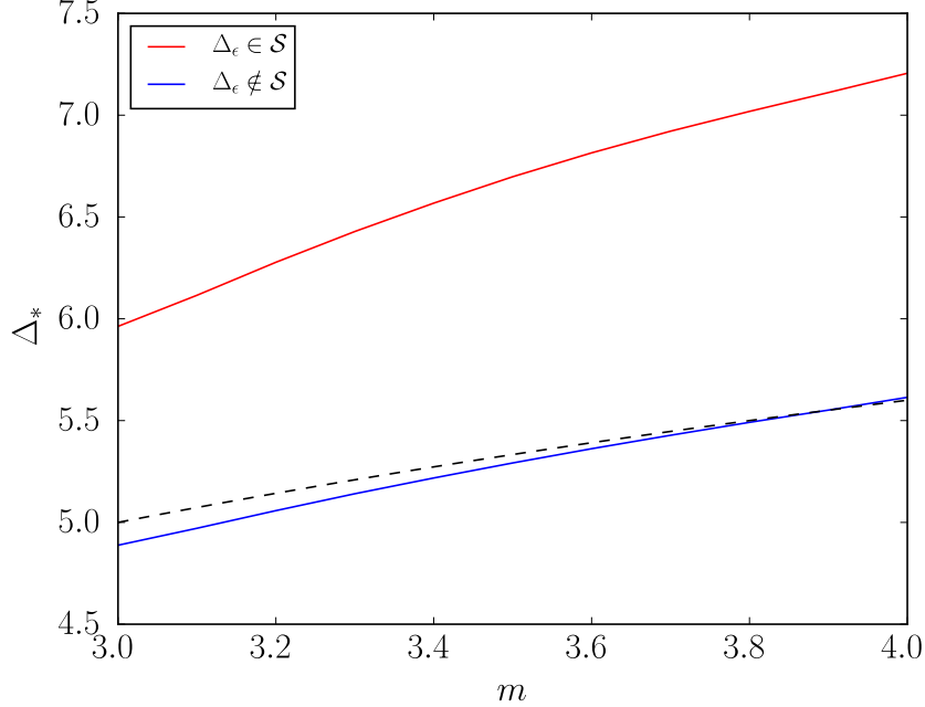
Figure 12: Dimension bounds for irrelevant operators in (3.60). The dotted line shows the dimension of the primary scalar \phi_{1,5} whose multiplet needs to be replaced for 3 < m < 4 .
