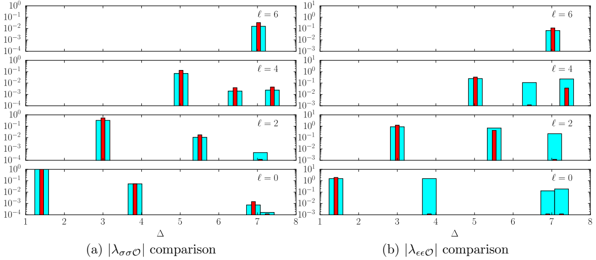
Figure 6: The analogue of Figure 5 for the 3D Ising model. In the fit, we have used the \mathbb{Z}_2 -even operator dimensions from [94]. This is already a longer list than anything that is likely to come from a one-correlator bootstrap. Due to a remaining bias in the spectrum, there is strong disagreement between the primal and dual methods.
