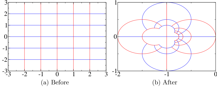
Figure 2: A set of grid lines and its image under the map e^{ib^\mu K_\mu} where b_\mu = (0, 1) . Clearly, the lines continue to meet at right angles.
