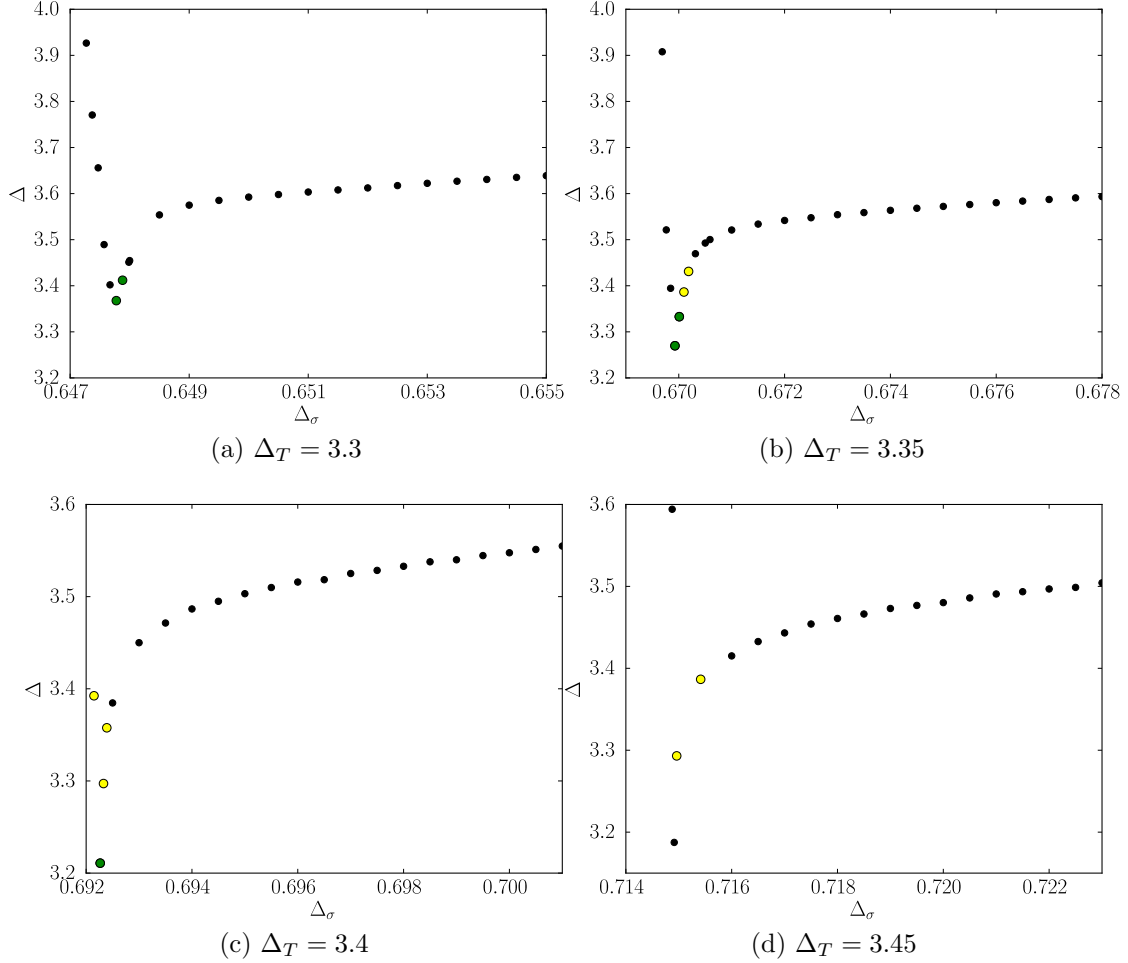
Figure 36: The dimension of the first irrelevant scalar in each of the four spectra extracted at the points shown in Figure 35. These have been taken from the \sigma \times \sigma , \epsilon \times \epsilon and \chi \times \chi OPEs as the scalars in \sigma \times \chi do not show an interesting feature. Points that are yellow and green respectively satisfy property 1 and property 2 as defined in the text. These points have also been made larger.
