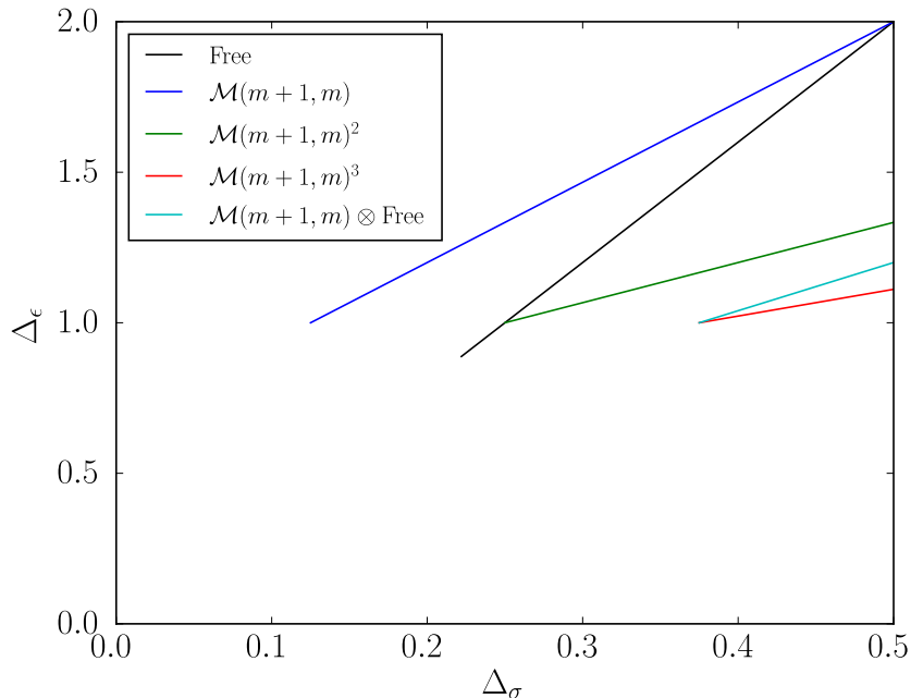
Figure 13: Tensor product theories that are allowed in both sides of Figure 8. Since we must have \Delta_\epsilon \geq 1 , all other tensor products involving the free field vertex operators necessarily lie to the right.
