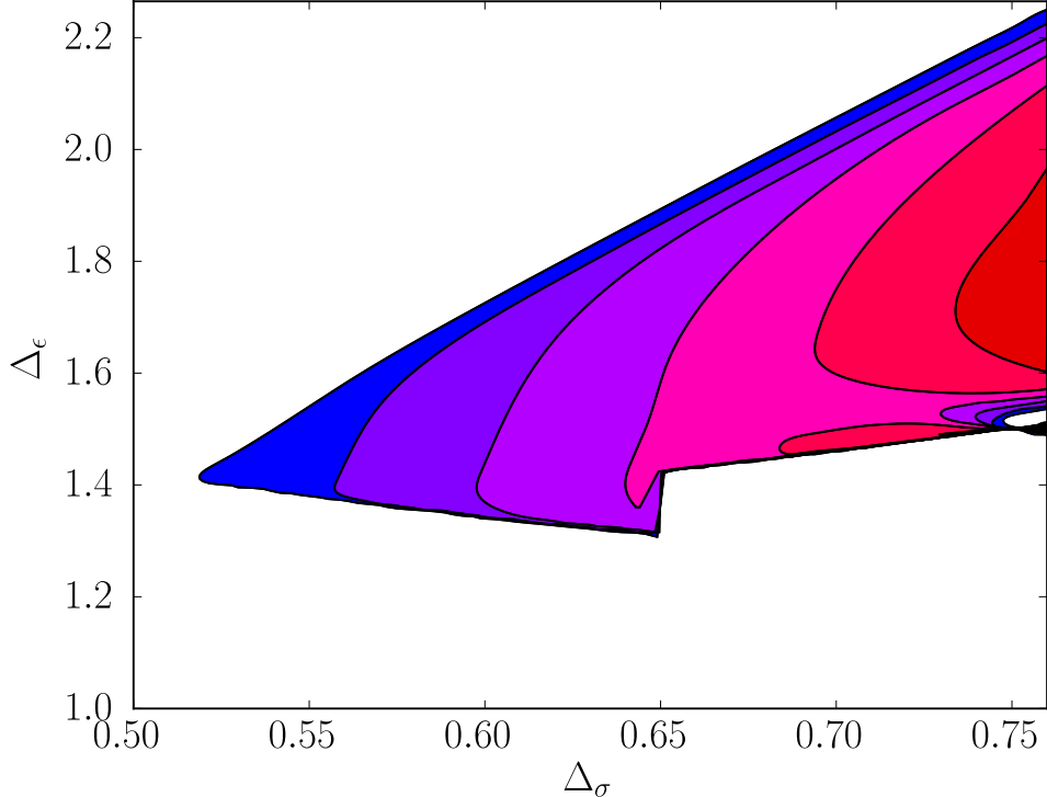
Figure 34: The allowed region in (\Delta_\sigma, \Delta_\epsilon) space found by imposing crossing symmetry and unitarity on the six correlator system that includes \sigma , \epsilon and \chi . As in Figure 32, the most permissive region (the blue one) allows the first \mathbb{Z}_2 -even spin-2 operator dimension \Delta_T to be as low as 3, while the most restrictive region (the red one) forces it to be at least 3.5. The other regions have \Delta_T \in \{3.1, 3.2, 3.3, 3.4\} . Derivative orders are (m_{\max}, n_{\max}) = (3, 5) . These regions account for protected double-twist operators in \sigma \times \chi and use ordinary conformal blocks which means that the \langle \sigma\sigma\chi\chi \rangle crossing equations are those of (4.156).
