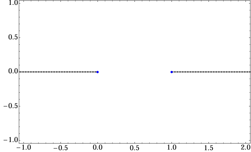
Figure 42: Continuing to complex z , our blocks have one branch cut from -\infty to 0 and another from 1 to \infty . This differs from higher-dimensional blocks which are analytic on \mathbb{C} \setminus (1, \infty) . As an example, we may multiply two SL(2; \mathbb{R}) blocks to get an SL(2; \mathbb{C}) block. This causes the left cut to cancel and the right cut to double.
