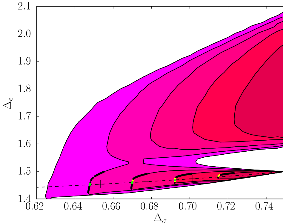
Figure 35: Five allowed regions whose spin-2 restrictions increment from \Delta_T \geq 3.25 on the left to \Delta_T \geq 3.45 on the right. They were found using ordinary conformal blocks with (m_{\max}, n_{\max}) = (5, 7) . Since no protected operators were assumed, the relevant crossing equation for \langle \sigma\sigma\chi\chi \rangle is (4.154). Green points contain the operator (\Delta, \ell) = (\Delta_T, 2) in all \mathbb{Z}_2 -even OPEs instead of just one of them. Green and yellow points contain a \mathbb{Z}_2 -even vector of dimension close to 6. All points that we have found to have neither property are marked in black. The perturbative dotted line shows \Delta_\epsilon as a function of \Delta_\sigma according to the Padé approximant in Table 16. Points on this line that are predicted to have \Delta_T \in \{3.3, 3.35, 3.4\} are denoted by crosses.
