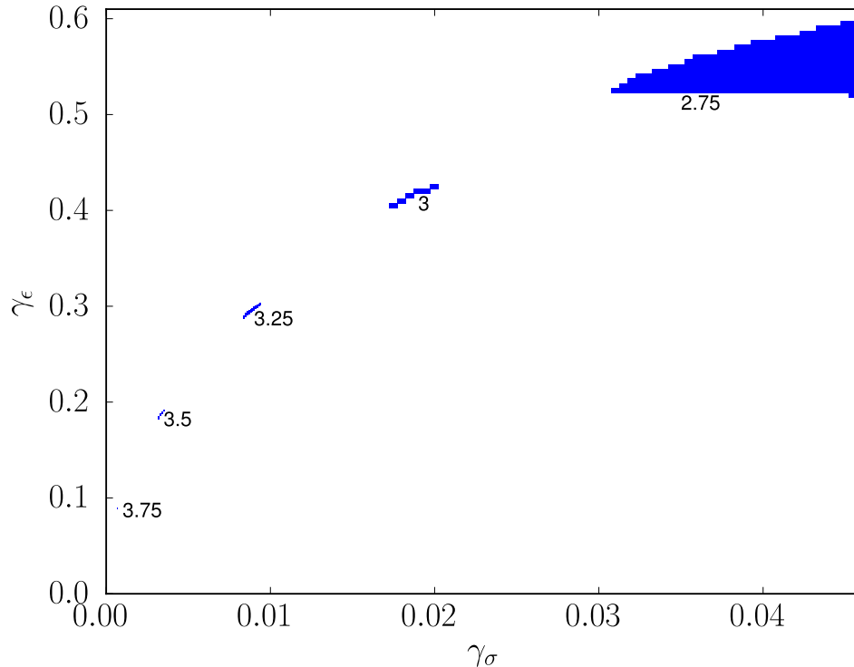
Figure 7: Allowed regions carved out by crossing symmetry and unitarity in a \mathbb{Z}_2 -symmetric system of correlators involving \sigma and \epsilon . Each value of d exhibits good agreement with the perturbative critical exponents of the Wilson-Fisher fixed-point.
