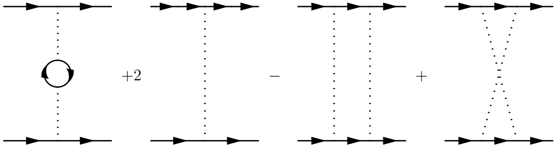
Figure 15: The one-loop correction to Figure 14. The two vertices in each diagram above should be summed over all g_n .
