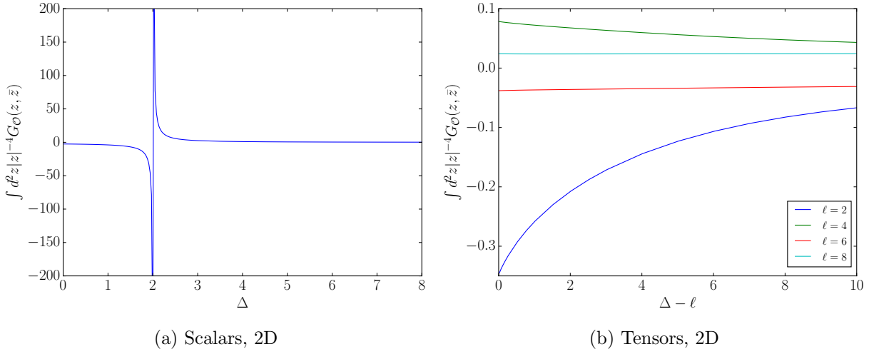
Figure 39: Plots showing how a primary operator in \hat{\mathcal{O}} \times \hat{\mathcal{O}} contributes to the beta function. These follow from a numerical integral but they may be obtained analytically in one dimension.
