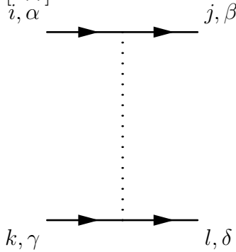
Figure 14: The diagram for a vertex which contracts fermion lines with g_n \delta_j^i \delta_l^k \left( \Gamma_A^{(n)} \right)_\beta^\alpha \left( \Gamma_A^{(n)} \right)_\delta^\gamma . Loop diagrams will of course introduce divergences which lead to a running of g_n .
