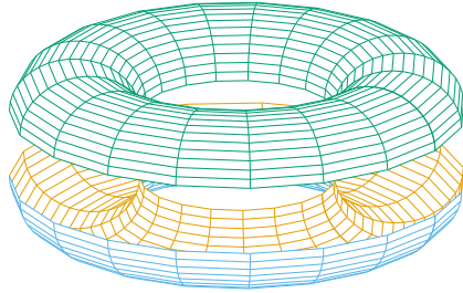
Figure 3: A torus in two halves, which are topologically equivalent to cylinders. If the same theory were defined on both halves, losing consistency after they are glued together would be a type of nonlocal behaviour.
