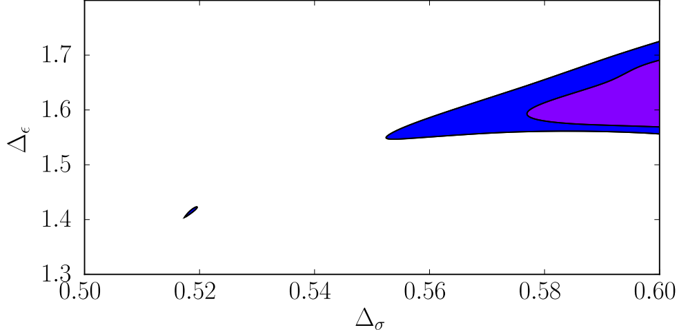
Figure 31: Constraints on the space of CFTs with one relevant primary operator of each parity. The allowed region for \Delta_T \geq 3 is blue, while the one for \Delta_T \geq 3.1 is purple. In the former case, an island around the 3D Ising model is separated from the rest of the region. This excludes many long-range Ising models which require \chi to be present.
