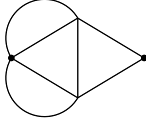
Figure 17: One of three two-loop diagrams that contributes to (4.12). Unlike the others, this one has only been computed recently.
