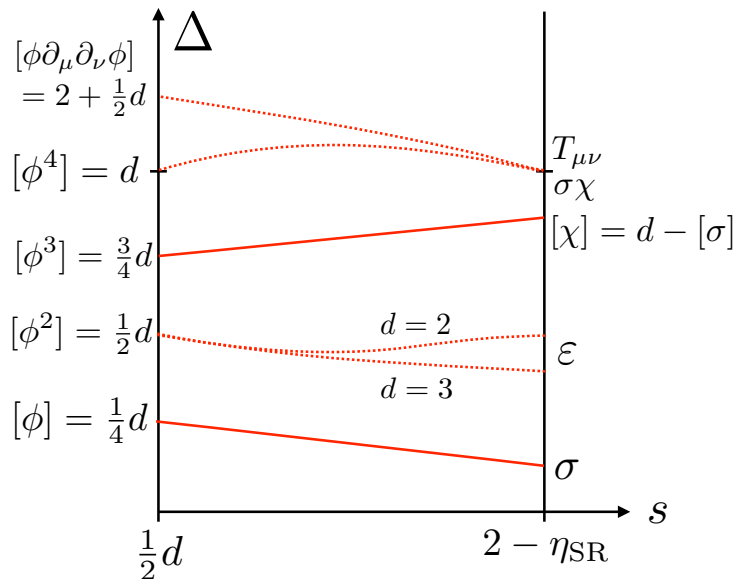
Figure 21: The dependence of dimensions of several important operators on s . The main text uses [\mathcal{O}] to denote the renormalized version of \mathcal{O} but here it is a shorthand for \Delta_{\mathcal{O}} .
