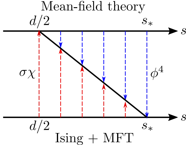
Figure 20: The RG flow diagram showing the two flows to the LRI where one is weakly coupled precisely when the other is strongly coupled.
