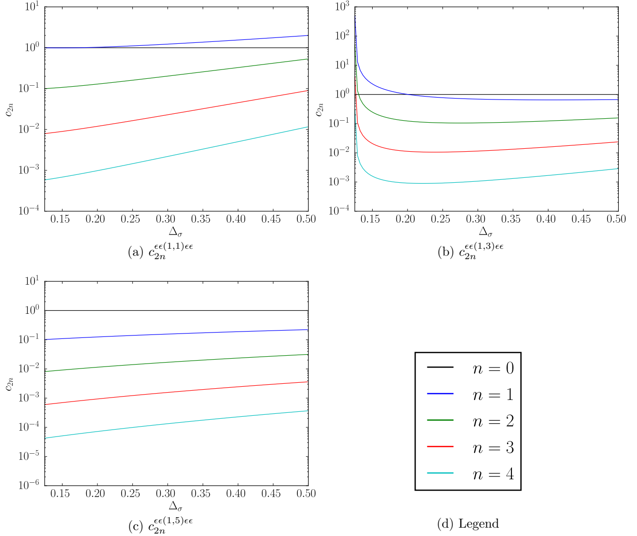
Figure 9: Log-scale plots of c_{2n}^{\epsilon\epsilon(1,s)\epsilon\epsilon} showing that the first five are all positive on the interval \frac{1}{8} \leq \Delta_\sigma \leq \frac{1}{2} .
