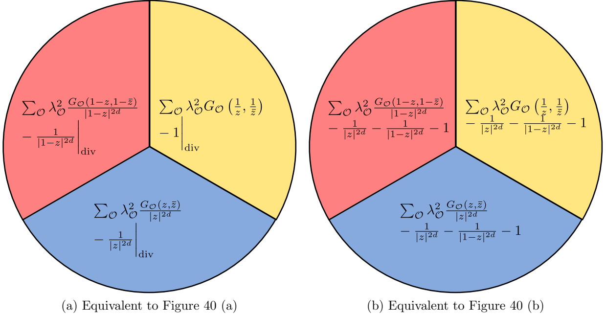
Figure 41: The cartoons obtained by splitting Figure 40 into s , t and u channel regions. In both cases, the identity block is not annihilated. A divergence subtraction is now no longer the same as a full subtraction. In particular, removing \text{div} everywhere in the left blob would not compute a physical quantity.
