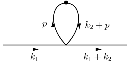
Figure 25: The T_{\mu\nu} operator, represented by a dot at the top with momentum flowing in, has its legs saturated by \phi .
