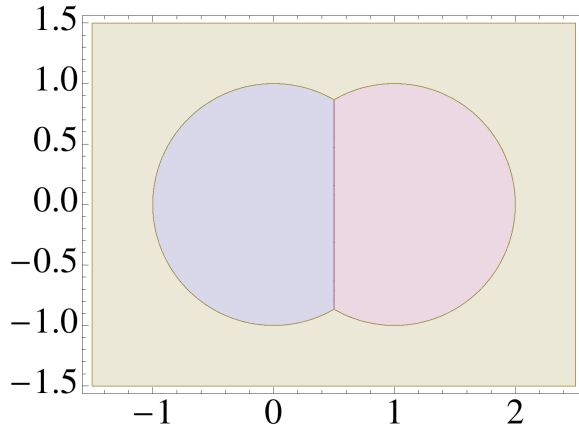
Figure 38: Once we send our four points to (0, z, 1, \infty) , \mathcal{R}_{12} , \mathcal{R}_{23} and \mathcal{R}_{13} map to the blue, red and yellow z -plane regions respectively. We have used a change of variables to give all integrals the blue domain, which we denote by \mathcal{R} .
