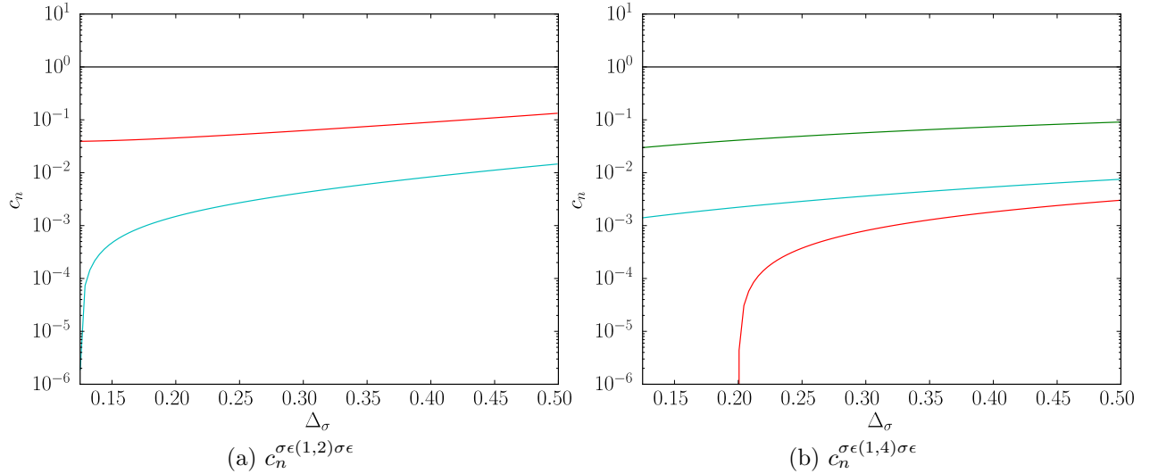
Figure 10: Log-scale plots of the c_n^{\sigma\epsilon(1,s)\sigma\epsilon} that are non-zero. The legend is the same as that of Figure 9.
