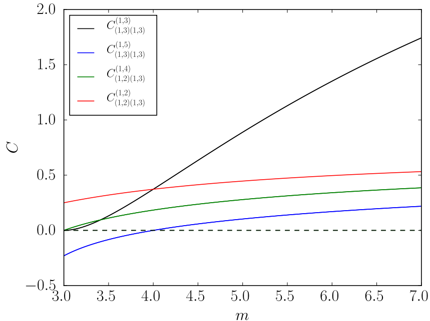
Figure 11: Low-lying squared OPE coefficients for Virasoro primaries in the generalized minimal models. Between the Ising model at m = 3 ( \Delta_\sigma = \frac{1}{8} ) and the tricritical Ising model at m = 4 ( \Delta_\sigma = \frac{1}{5} ), there is one that becomes negative.
