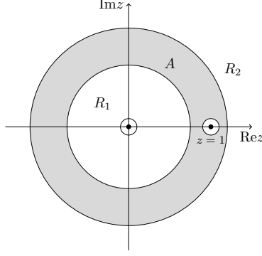
Figure 23: The three integration regions (4.85).
