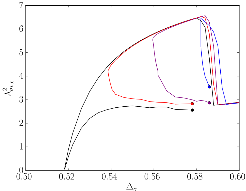
Figure 33: The bound on \lambda_{\sigma\epsilon\chi}^2 as a function of \Delta_\sigma computed for (m_{\max}, n_{\max}) = (5, 7) . The minimum \Delta_T is 3 for the black line, 3.05 for the red line, 3.1 for the purple line and 3.15 for the blue line. The OPE coefficient is maximized along the upper and lower branches of Figure 32. However, we have chosen not to go all the way to \Delta_\sigma = 0.6 along the upper branch. Doing so would yield several intersecting lines that reduce visual clarity.
