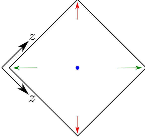
Figure 1: Important limits for the cross-ratios starting from 0 < z, \bar{z} < 1 . The numerical bootstrap is usually conducted with reference to the blue point (z, \bar{z}) = (\frac{1}{2}, \frac{1}{2}) , even though it works for any Euclidean configuration. The red arrows denote the lightcone limit in which the operator product expansion (OPE) becomes an expansion in twist. This leads to a universal structure in the large spin sector of a CFT [36–39]. The green arrows denote the deep Euclidean limit which controls the sector with large scaling dimension. The leading estimates in [40, 41] have recently been improved through the use of complex tauberian theorems [42, 43]. Not shown in the figure is the so called Regge limit which involves the second sheet and provides an analogue of high energy scattering [44–48].
