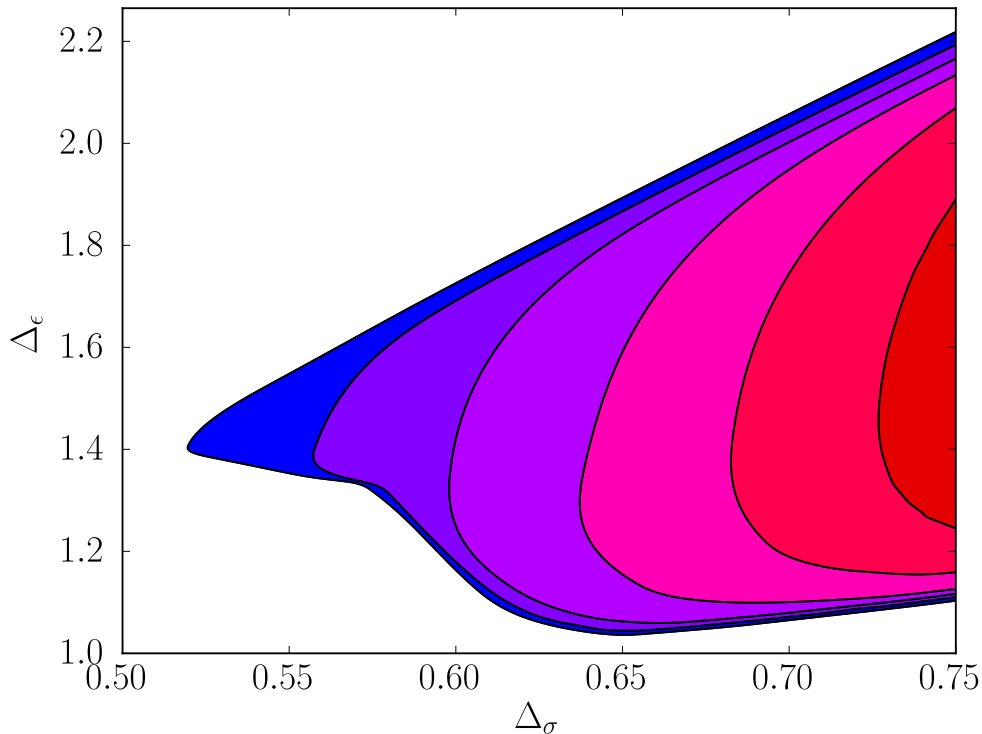
Figure 32: A multi-correlator version of Figure 29, computed with (m_{\max}, n_{\max}) = (3, 5) . The upper bounds are similar to the ones plotted before but the lower bounds are new. We have plotted them using a simple bisection while also testing interior points to ensure that there are no holes. Again, blue signifies \Delta_T \geq 3 and red signifies \Delta_T \geq 3.5 .
