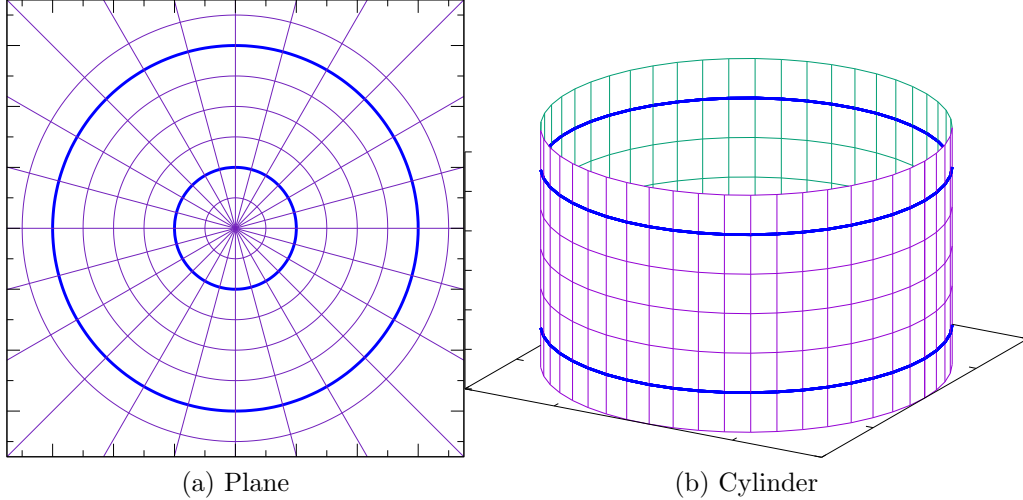
Figure 4: The plane and the cylinder showing a mapping between circles at fixed r and fixed t . States on the right live on these circles while local operators on the left live at points. We learn two interesting things from the fact that D = r\partial_r maps to H = \partial_t . The first is that the spectrum of scaling dimensions must be bounded from below in a unitary theory. The second is a general expectation that D (unlike the plane Hamiltonian) should have a discrete spectrum.
