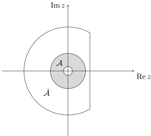
Figure 22: The integration region \mathcal{R} .
