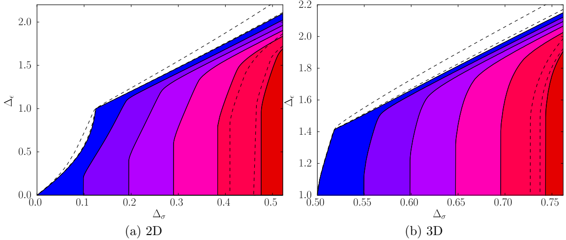
Figure 29: The upper bound on \Delta_\epsilon as a function of \Delta_\sigma . Our spin-2 constraint goes from \Delta_T \geq d (blue) to \Delta_T \geq \frac{d}{2} + 2 (red) in evenly spaced steps. Again, our main plots have (m_{\max}, n_{\max}) = (7, 9) with dotted lines for (5, 7) and (3, 5) . As expected, the convergence of the red region is slower than that of the blue region.
