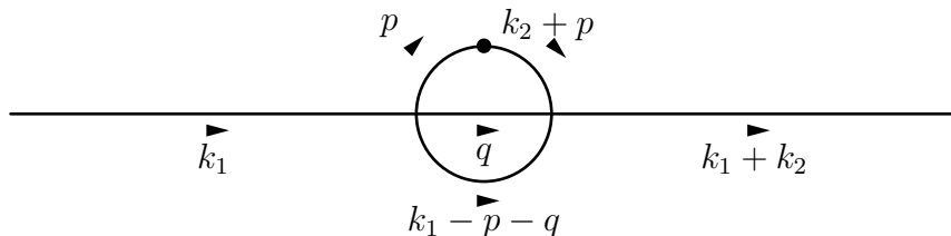
Figure 26: The most interesting two-loop contribution to \langle\phi\phi T\rangle .
