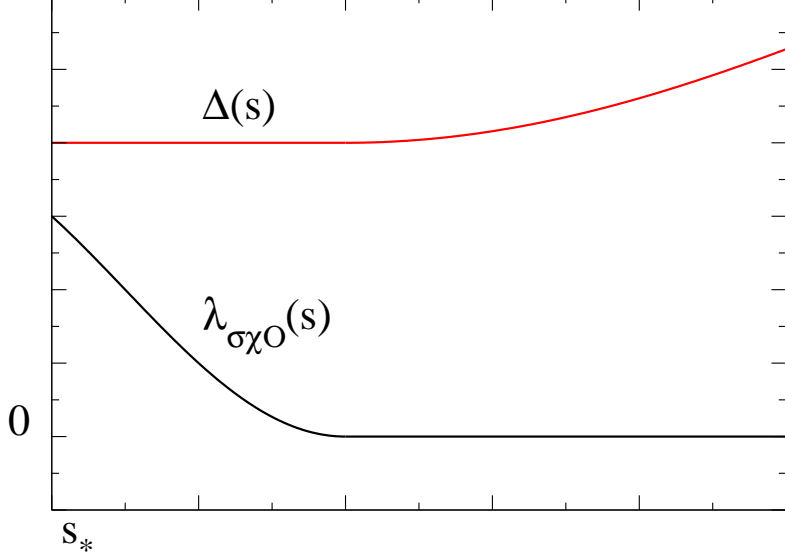
Figure 27: A possible way out of our non-renormalization theorem for odd-spin primary operators in \sigma \times \chi . The strongest statement we can make is that their dimensions are protected in an open neighbourhood of any point where \lambda_{\sigma\chi\mathcal{O}}^2 > 0 . It could be the case that at least one renormalizes after decoupling at an intermediate value of s .
