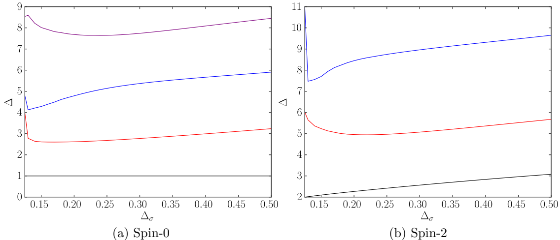
Figure 30: A few scaling dimensions in the extremal spectrum having maximal \lambda_{\sigma\sigma\epsilon}^2 with \Delta_\epsilon = 1 . These are zeros of the functional that is found during the maximization procedure. For all of the spins that we have tested, it is plausible that these could approximate primary operators in the LRI.
