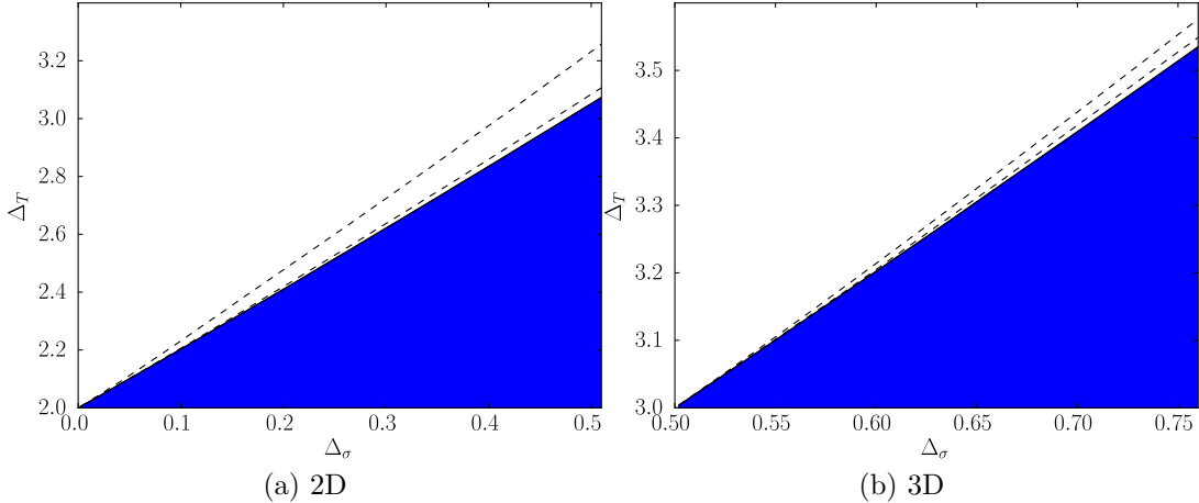
Figure 28: The allowed region for the first spin-2 operator dimension \Delta_T as a function of \Delta_\sigma . In both 2D and 3D, the bound appears to be converging to \Delta_T = 2\Delta_\sigma + 2 . The blue region was obtained with (m_{\max}, n_{\max}) = (7, 9) while (5, 7) and (3, 5) are shown for comparison.
