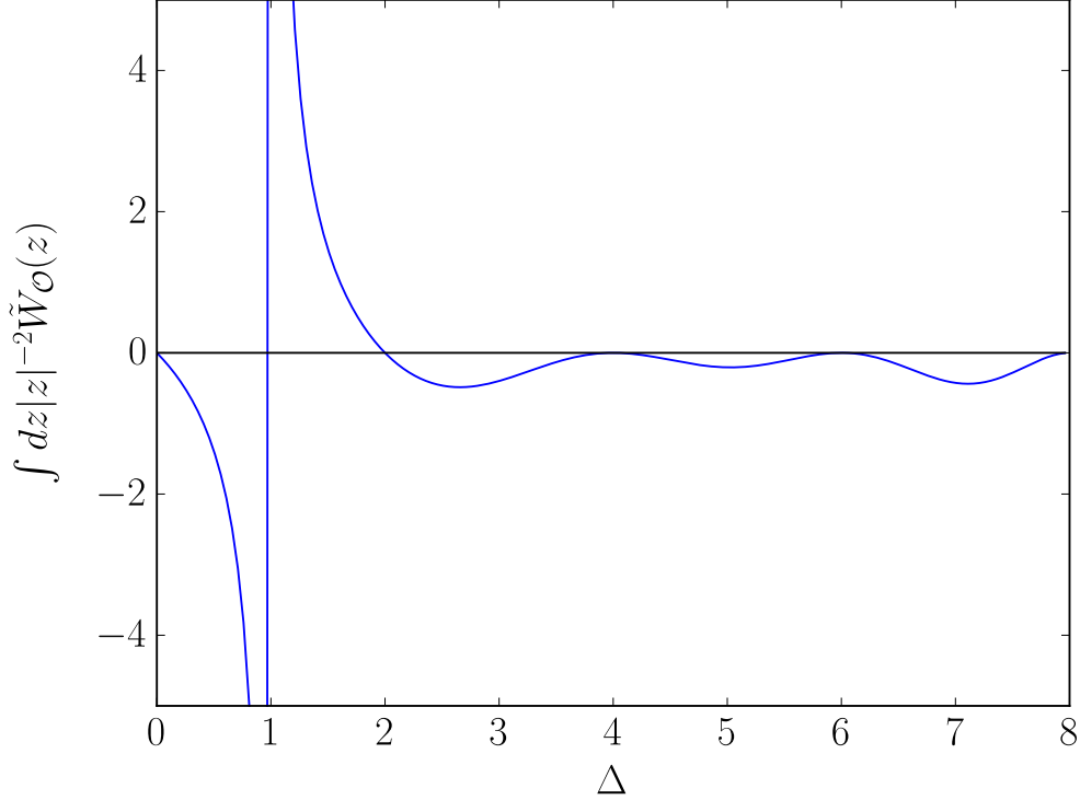
Figure 43: The regulated integral of a Polyakov block as a function of \Delta for \Delta_\phi = 1 . Due to the zeros at double-twist dimensions, which are mostly second-order, this function has exactly the same form as the action of an extremal functional for the gap \Delta = 2 . It would be interesting to check that the numerical bootstrap is returning this functional multiplied by -1 .
